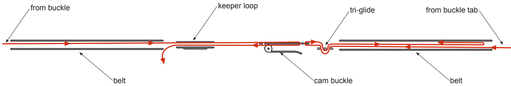
Grillslinger Webbing Arrangement Sectional Diagram Not to Scale
